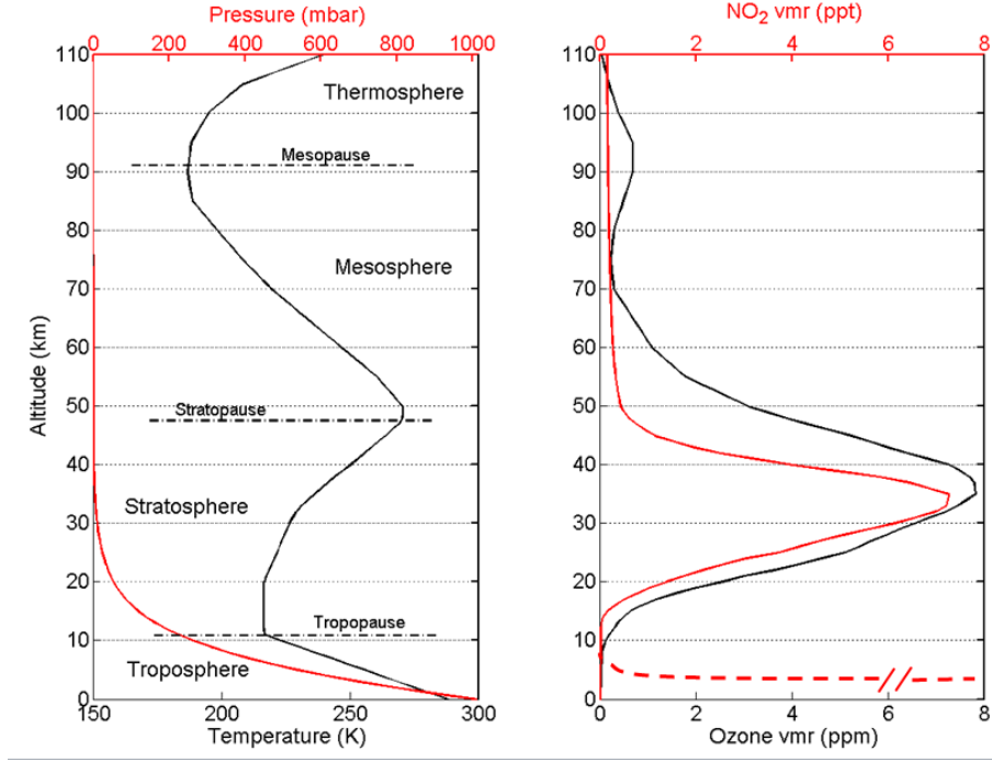
Figure 2.3: Vertical structure of a standard atmosphere (Anderson et al., 1986). The different layers are defined according to the temperature gradient. The right panel shows standard ozone and \text{NO}_2 profiles. Real profiles vary with time and location, in particular, for the \text{NO}_2 , the tropospheric contribution (red dashed curve) may dominate the total column.
