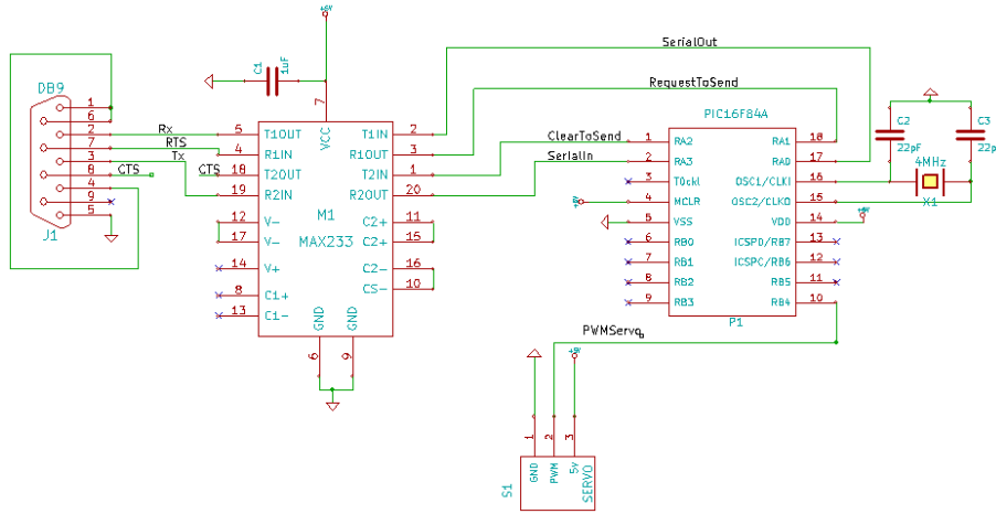
Figure 8.5: Electronic scheme of the scanning mechanism.
