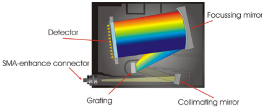
Figure 4.5: Schematic of the Avantes spectrometer used for ULM-DOAS, Mobile-DOAS, and SWING, from www.avantes.com .
