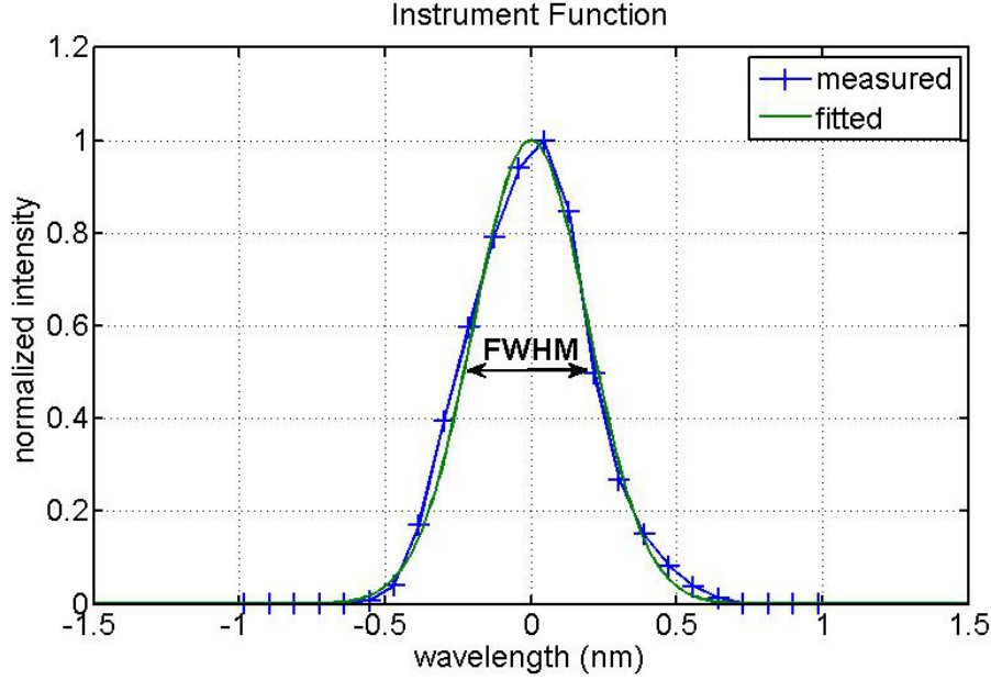
Figure 4.8: Instrument function of the ALS-DOAS instrument measured with an Hg-Cd lamp at 404.7 nm and fitted as a Gaussian using QDOAS. The crosses in the measured function indicate the pixel centers.
