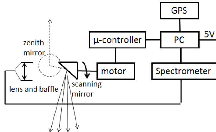
Figure 8.4: Scheme of the SWING payload.
