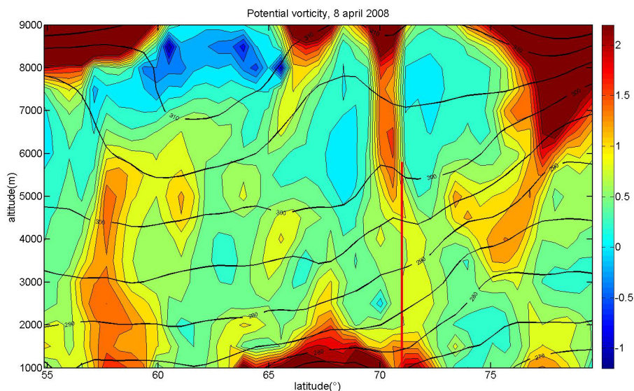
Figure 5.16: Potential vorticity on 8 April 2008
