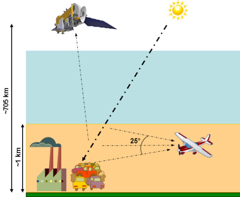
Figure 6.1: Geometry of our ULM-DOAS measurements compared to a nadir-looking satellite instrument like OMI.
