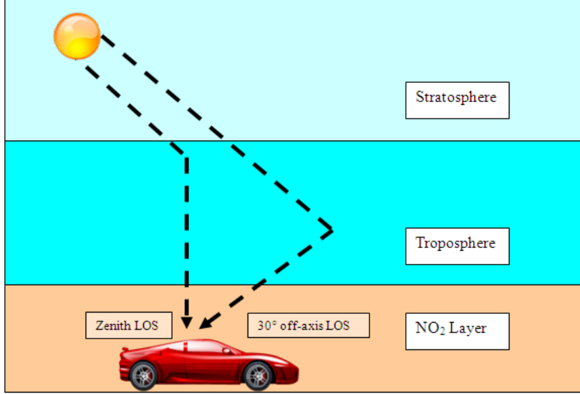
Figure 7.1: Geometry of the Mobile-DOAS measurements.
