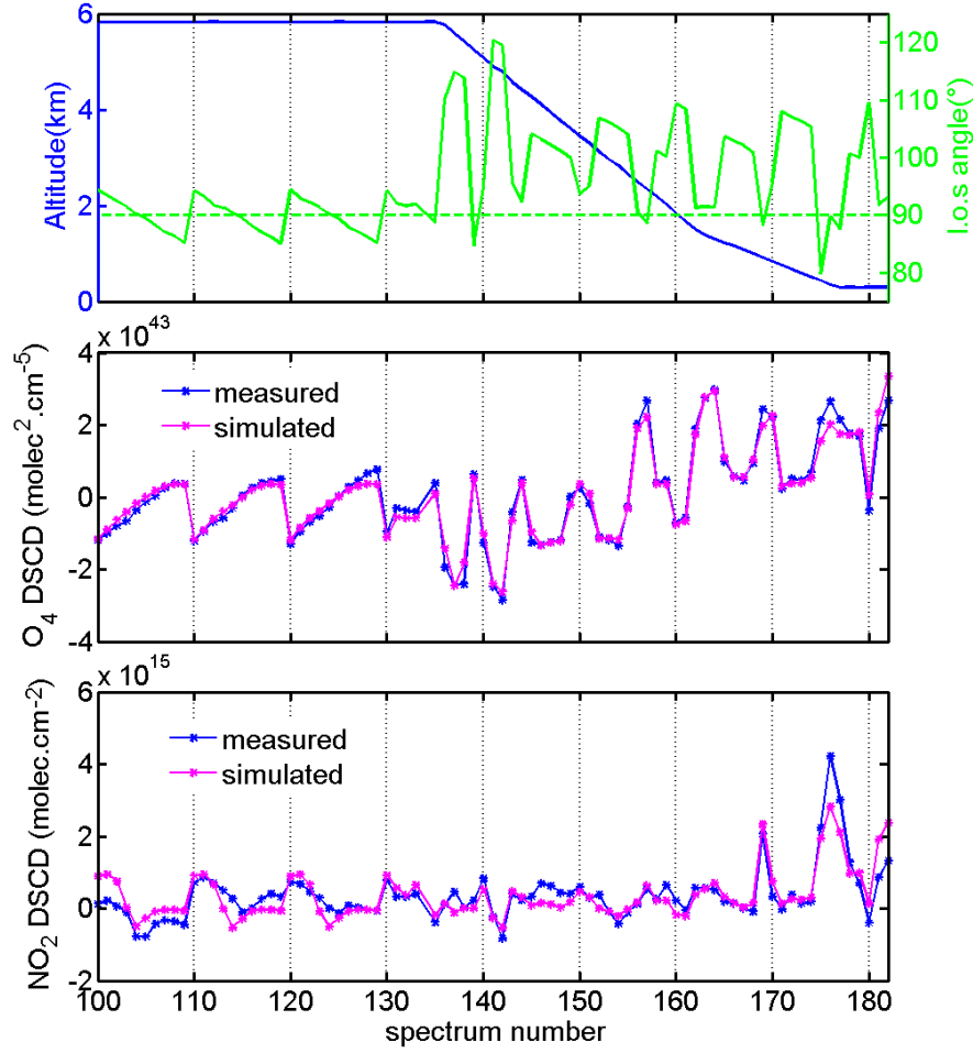
Figure 5.9: DSCD measurements during the as0831 flight (8 April 2008). The upper panel shows the plane altitude (blue) and the telescope line-of-sight angle (green, 0^\circ is nadir, 90^\circ horizontal). On the middle and bottom panels, measured DSCD, respectively of O_4 and NO_2 , are compared with simulations. Oscillations on the DSCD series are caused by the telescope scanning. Discrepancies between measured and simulated DSCD are larger in the boundary layer, where true aerosol extinction and NO_2 concentration are different from the model.
