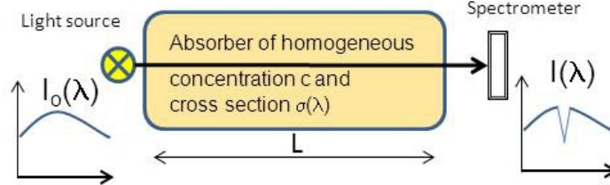
Figure 3.1: Absorption spectroscopy in the lab.
