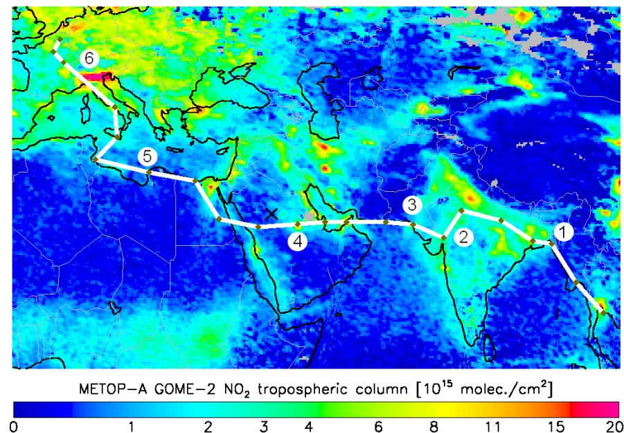
Figure 6.4: Flight tracks of the Earth Challenge expedition on a NO 2 GOME-2 map. The numbers correspond to the measurements presented in this paper: (1) Chittagong (Bangladesh, 4 November 2009), (2) Rajasthan (India, 15 November 2009), (3) Karachi (Pakistan, 16 November 2009), (4) Riyadh (Saudi Arabia, 24 November 2009), (5) Benghazi (Libya, 27 November 2009), (6) Po Valley (Italy, 2 December 2009). The cross west of Riyadh indicates a sand storm (see section 6.5.3).
