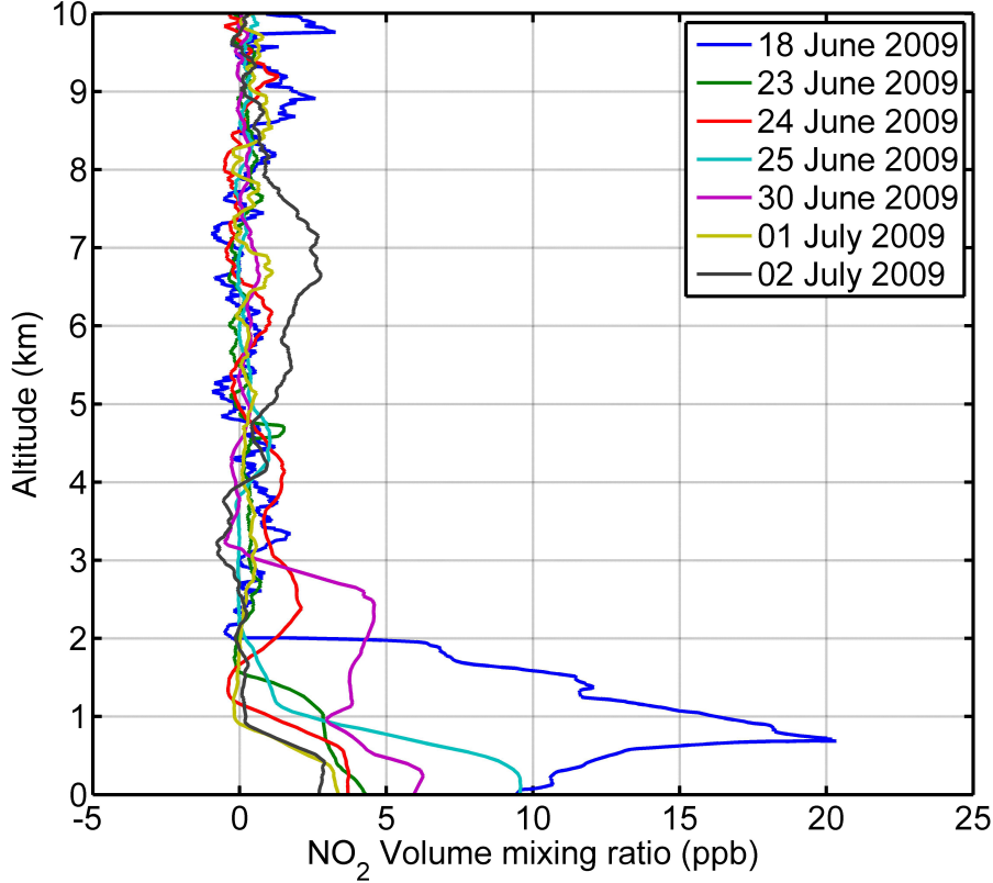
Figure 2.9: In-situ tropospheric \text{NO}_2 profiles during CINDI campaign.
