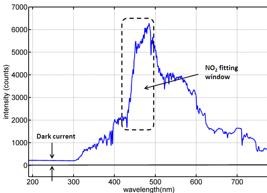
Figure 4.10: Typical spectrum of scattered sky light as recorded by the Avantes spectrometer. The signal between 200 and 250 nm is used to estimate the bias.
