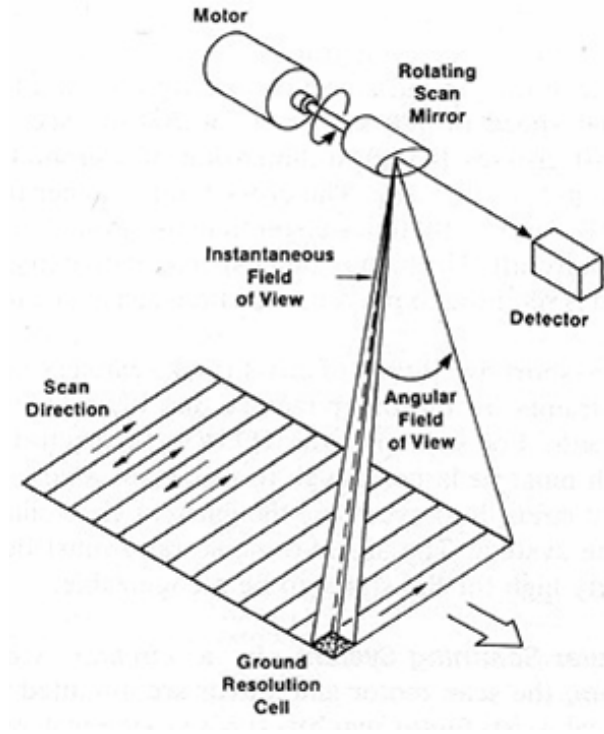
Figure 8.1: Principle of whiskbroom imaging (Sabins, 1997).
