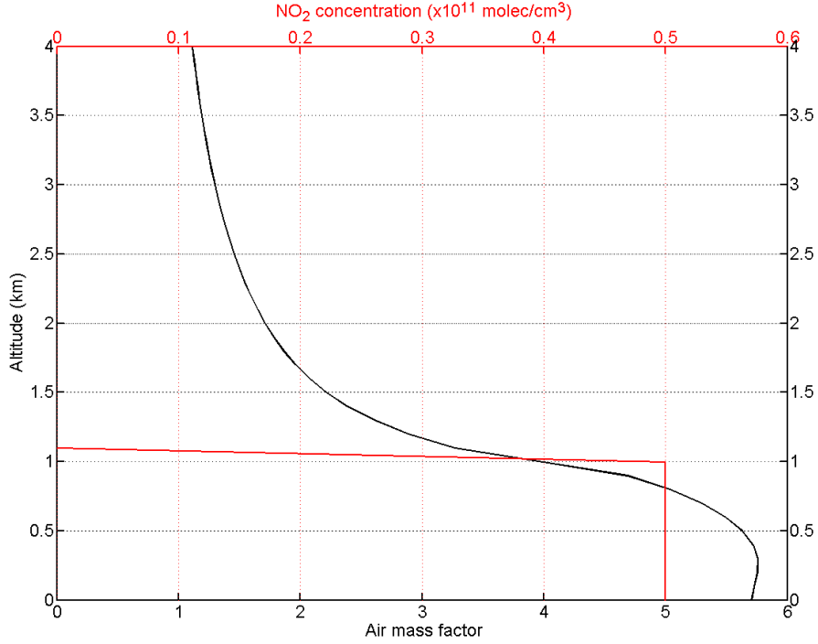
Figure 6.7: Air mass factor versus altitude (black) for an idealized \text{NO}_2 tropospheric profile (red) well mixed in the boundary layer and of negligible concentration in the free troposphere. The calculations were done at 460 nm, setting an albedo of 0.1, a relative azimuth and solar zenith angle of 90^\circ and 45^\circ , respectively, and a surface visibility of 20 km.
