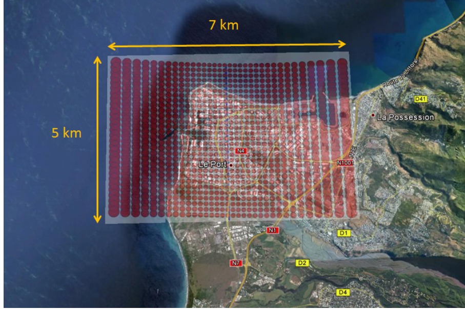
Figure 8.2: Ground cover for a flight altitude of 3 km and an angular field of view of 100^\circ .
