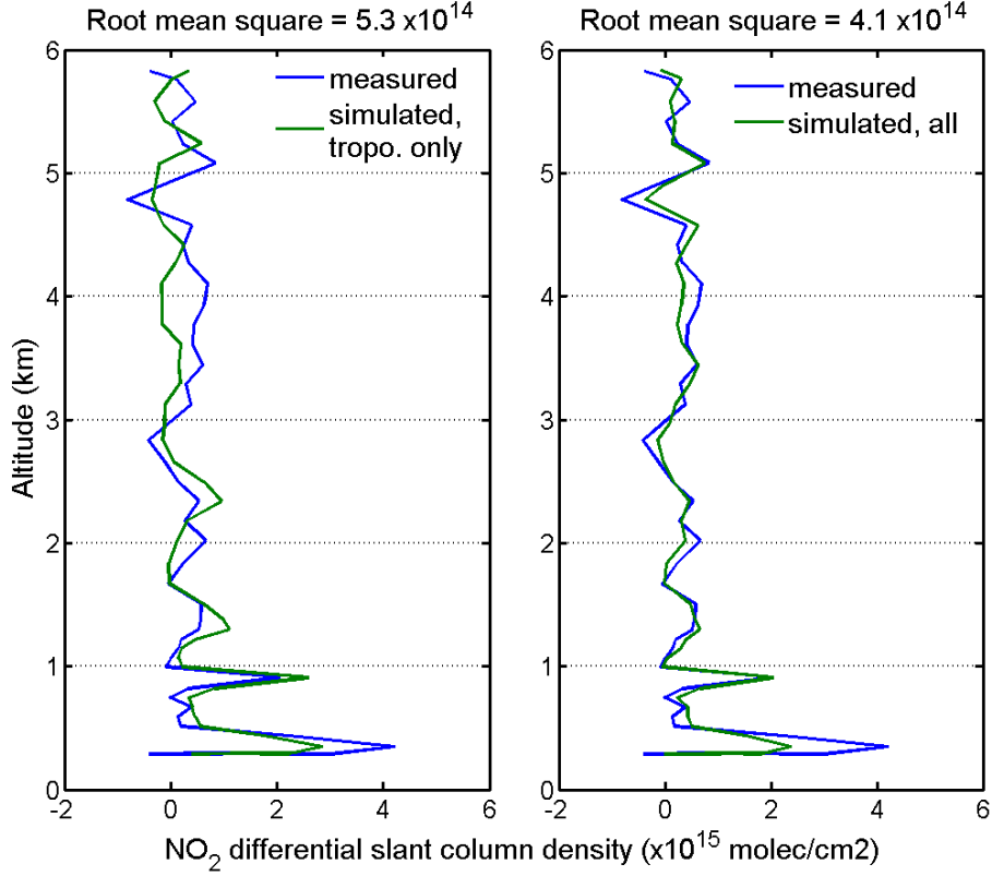
Figure 5.10: Influence of the stratosphere on \text{NO}_2 tropospheric observations. Measured \text{NO}_2 DSCD during the sounding (blue) are compared with simulations (green) neglecting the stratosphere (left) or not (right). The latter agrees better with the observations.
