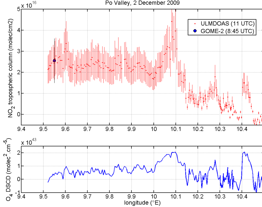
Figure 6.11: ULM-DOAS (red) and GOME-2 (blue) measurements over Italy (2 December 2009). ULM-DOAS data were recorded between 10:29 and 12:14 UTC and cover the latitude range from 44.58^\circ to 45.54^\circ . The zone west of 10^\circ E is the Po Valley.
