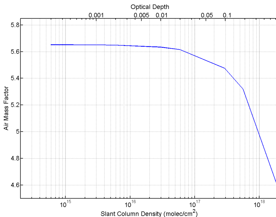
Figure 6.9: Air mass factor versus slant column density. \text{NO}_2 loading starts to influence significantly the radiative transfer above 5 \times 10^{16} \text{ molec/cm}^2 . The calculations were done at 460 nm for an altitude of 0.5 km, setting a relative azimuth and solar zenith angle of 90^\circ and 45^\circ , respectively, and with a 1 km thick homogeneous boundary layer.
