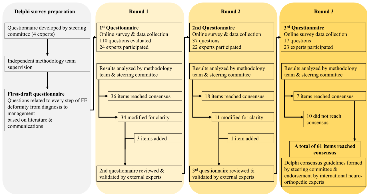
Fig. 1. Delphi process.
