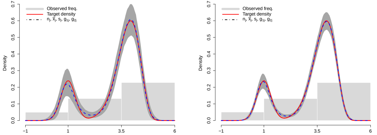
Figure 3: Simulation study – Connected pointwise intervals containing 95% of the estimated densities over the S = 500 datasets and obtained using tabulated summary statistics \mathcal{D}_4 over J = 3 classes. Left panel: n = 250 ; Right panel: n = 1000 .
