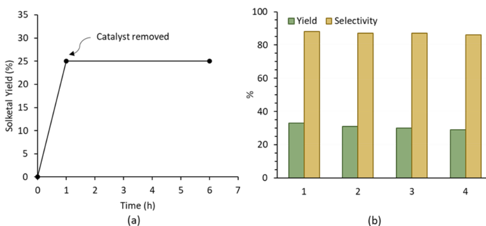
Figure 8 – Hot filtration test (Ga leaching test). Conditions: 1 h, 50 °C, Gly: Ac = 1: 4, 600 \mu L EtOH, 10 mg catalyst. The catalyst was removed from the mixture after 1h by centrifugation and let it reacted in the same conditions for 5 supplementary hours. (a) and recycling test. Conditions: 1 h, 50 °C, Gly: Ac = 1: 4 (b) on Ga-NS. Conversion estimated via ^1\text{H} NMR of the reaction mixture.
