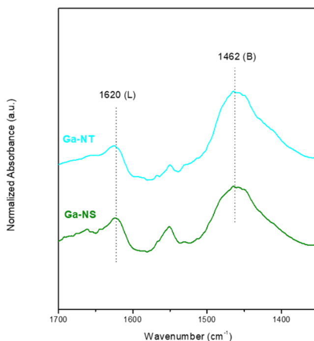
Figure 5 - Difference FT IR spectra of ammonia dosages on Ga-NT after outgassing at 400 °C (spectrum of the bare outgassed sample has been subtracted). L and B mean Lewis and Brønsted, respectively
