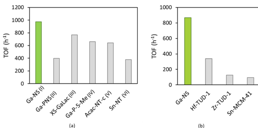
Figure 9 – Comparison of Ga-NS with catalysts from literature: (a) tested in the following conditions: 50 °C, 10 mg of catalyst, Gly: Ac = 1 (0.01 mol): 4, 2 h. (I)[48], (II)[9], (III)[37], (IV)[13] (V).[61] (VI) 80 °C, 10 mg of catalyst, Gly: Ac = 1 (0.01 mol): 1, 1 h, 1.48 g of tert-butanol. The TOF of Hf-TUD-1, Zr-TUD-1 and Sn-MCM-41 were calculated based on data extrapolated from the kinetic.[36]
