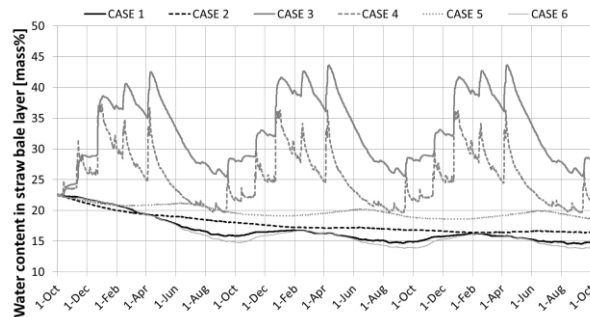
Figure 3: Series A1: Water content evolution in straw bale.
