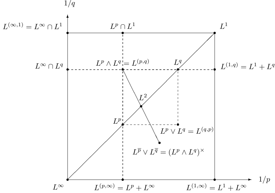
Figure 1: The unit square describing the lattice \mathcal{J} .
