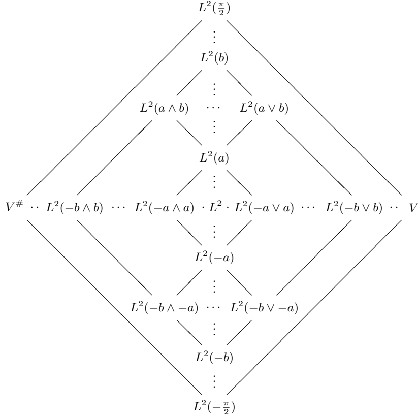
Figure 4: The van Winter LHS.
