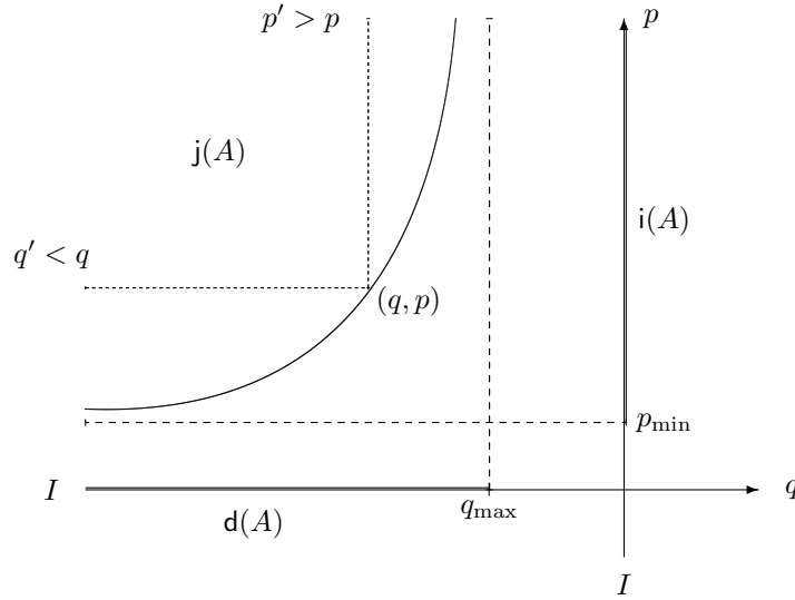
Figure 2: Characterization of the operator A , in the case of a scale.
