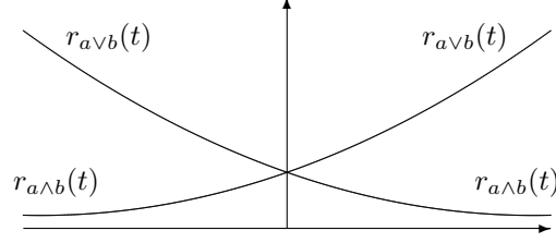
Figure 3: The functions r_{a \wedge b} and r_{a \vee b} for a < 0 < b .
