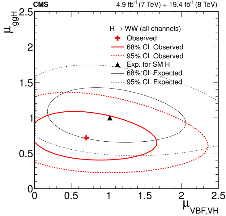
Figure 25. Likelihood profiles on \mu_{\text{ggH}} and \mu_{\text{VBF,VH}} at 68% (solid) and 95% CL (dotted). The expected (black) and observed (red) distributions for m_{\text{H}} = 125.6 \text{ GeV} are shown.
