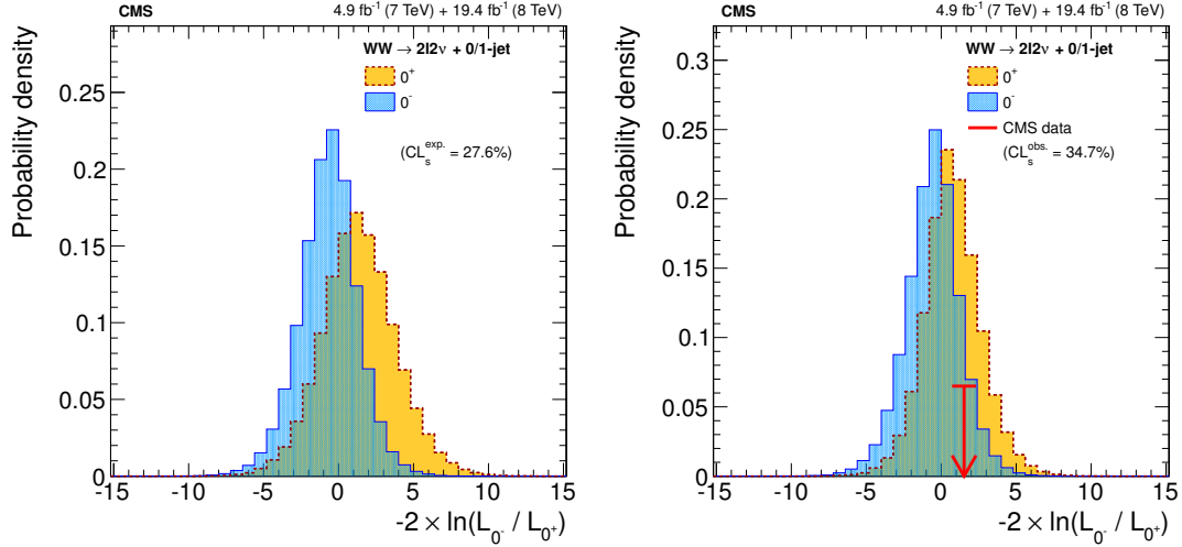
Figure 30. Distributions of -2 \ln(L_{0^-}/L_{0^+}) , combining the 0-jet and 1-jet categories in the e\mu final state, for the 0^+ and 0^- hypotheses at m_H = 125.6 GeV. The distributions are produced assuming \sigma/\sigma_{SM}=1 (left) and using the signal strength determined from the fit to data (right). The observed value is indicated by the red arrow.
