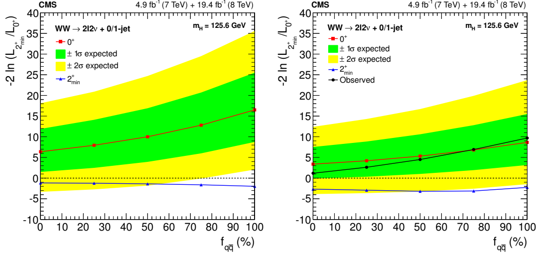
Figure 29. Median test statistic for the 0^+ and 2_{min}^+ hypotheses, as a function of f_{q\bar{q}} of the 2_{min}^+ particle, assuming \sigma/\sigma_{SM} = 1 (left) and using the \sigma/\sigma_{SM} value determined from the fit to data (right). The observed values are also reported in the second case.
