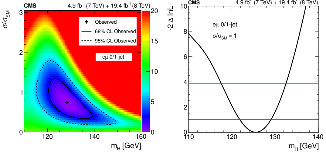
Figure 24. Confidence intervals in the (\sigma/\sigma_{\text{SM}}, m_H) plane using the parametric unbinned fit in (m_R, \Delta\phi_R) distribution (left) for the 0-jet and 1-jet categories in the e\mu final states. Solid and dashed lines indicate the 68% and 95% CL contours, respectively. On the right, the one-dimensional likelihood profile for \sigma/\sigma_{\text{SM}}=1 is shown. The crossings with the horizontal line at -2\Delta \ln L = 1 (3.84) define the 68% (95%) CL interval. The SM Higgs boson production cross section uncertainties are considered.
