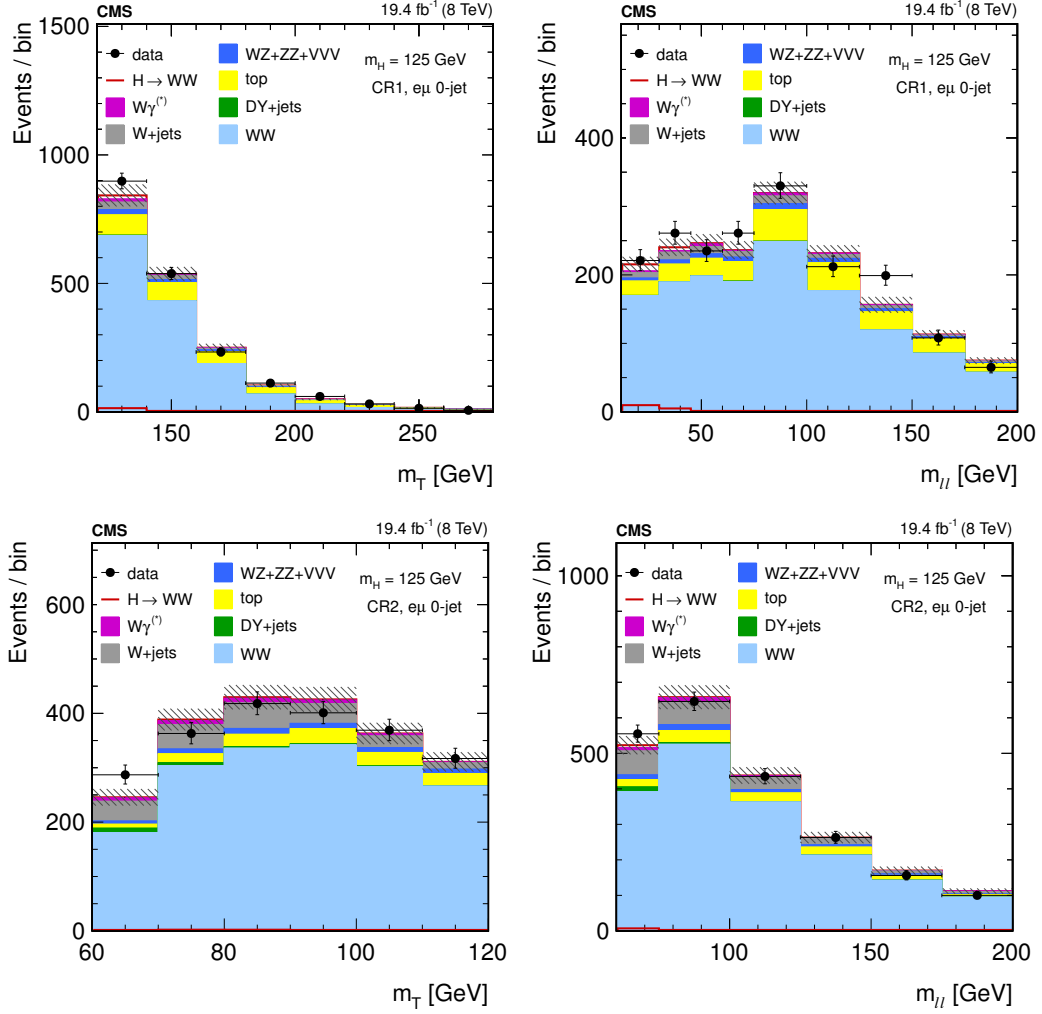
Figure 11. Distributions of m_T (left) and m_{\ell\ell} (right) extrapolated to the control regions CR1 (top) and CR2 (bottom) in the 0-jet bin category, after fitting the other control region.
