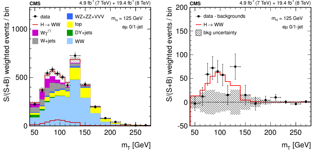
Figure 7. The m_T distribution in the e\mu final state for the 0-jet and 1-jet categories combined for observed data superimposed on signal + background events and separately for the signal events alone (left) and background-subtracted data with best-fit signal component (right). The signal and background processes are normalized to the result of the template fit to the (m_T, m_{\ell\ell}) distribution and weighted according to the observed S/(S+B) ratio in each bin of the m_{\ell\ell} distribution integrating over the m_T variable. To better visualize a peak structure, an extended m_T range including m_T=[40,60] GeV is shown, with the normalization of signal and background events extrapolated from the fit result.
