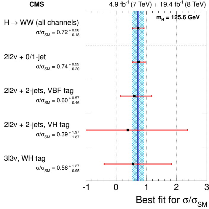
Figure 23. Observed \sigma/\sigma_{\text{SM}} for m_H = 125.6 \text{ GeV} for each category used in the combination. The observed \sigma/\sigma_{\text{SM}} value in the \text{ZH} \rightarrow 3\ell\nu 2 jets category is 6.41^{+7.43}_{-6.38} . Given its relatively large uncertainty with respect to the other categories it is not shown individually, but it is used in the combination.
