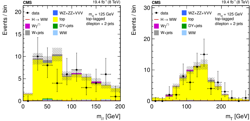
Figure 36. The m_{\ell\ell} (left) and m_T (right) distributions in the 2-jet category for top-tagged events after applying the WW and VBF-tag selections for the \sqrt{s} = 8 TeV data sample. The uncertainty band includes the statistical and systematic uncertainty for all background processes.
