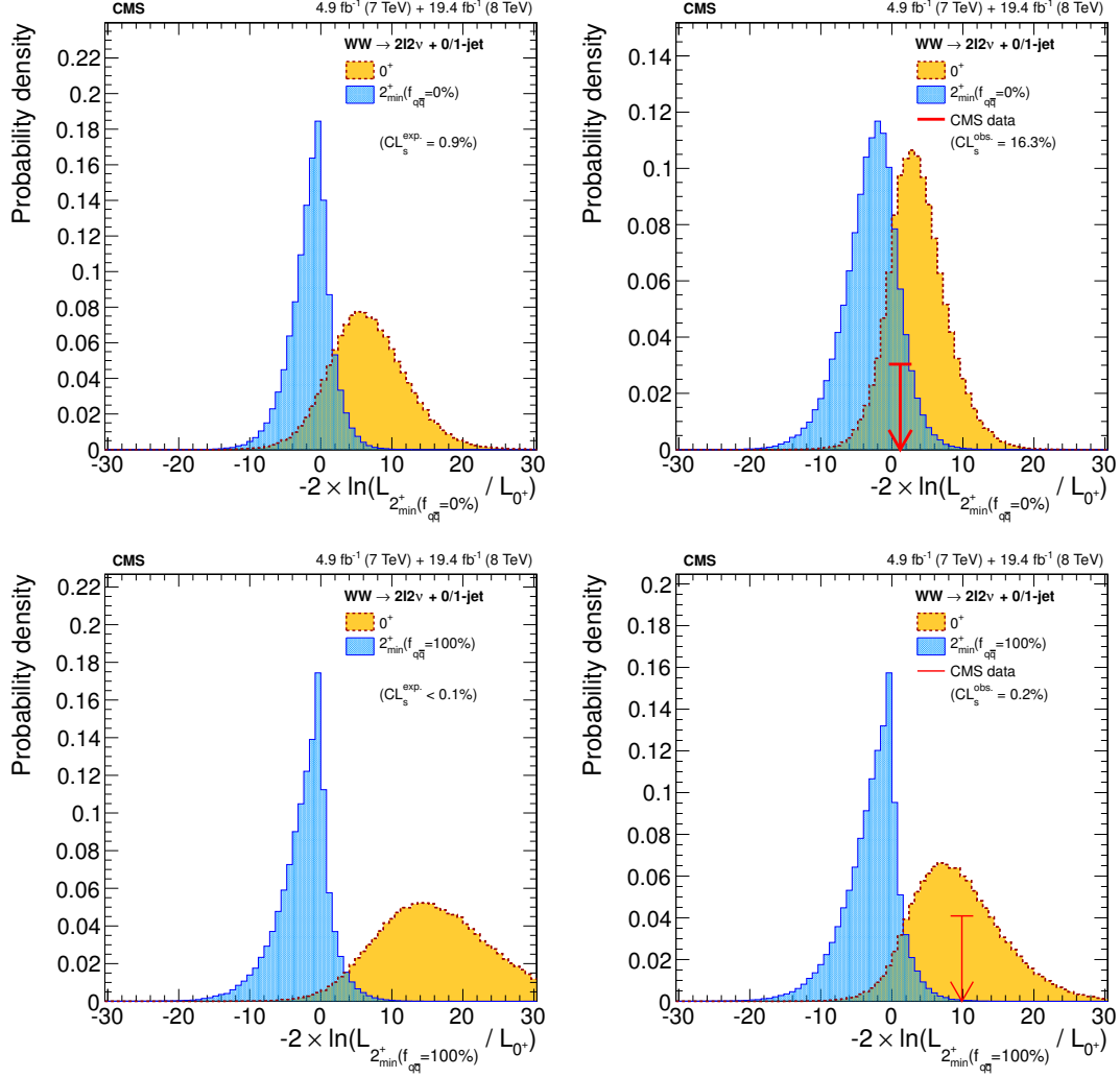
Figure 28. Distributions of -2 \ln(L_{2_{min}^+}/L_{0^+}) , combining the 0-jet and 1-jet categories in the e\mu final state, for the 0^+ and 2_{min}^+ hypotheses at m_H = 125.6 GeV. The distributions are produced assuming \sigma/\sigma_{SM}=1 (left) and using the \sigma/\sigma_{SM} value determined from the fit to data (right). The distributions are shown for the case f_{q\bar{q}}=0\% (top) and f_{q\bar{q}}=100\% (bottom). The observed value is indicated by the red arrow.
