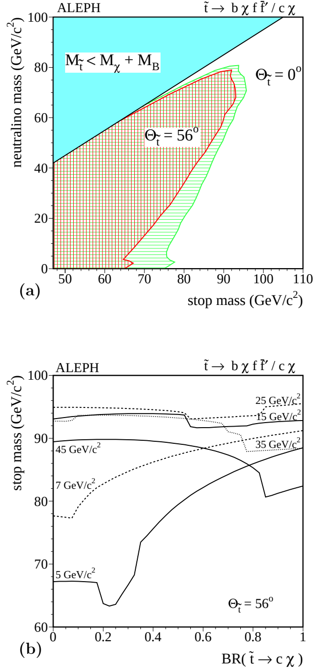
Figure 4: (a) Branching ratio independent excluded regions at 95% C.L. in the M_{\tilde{\chi}} vs M_{\tilde{t}} plane, from \tilde{t} \rightarrow b \chi f \tilde{f}' and \tilde{t} \rightarrow c \chi searches. The excluded regions are given for \theta_{\tilde{t}} = 0^\circ , corresponding to maximum \tilde{t}\tilde{t}Z coupling, and for \theta_{\tilde{t}} = 56^\circ , corresponding to vanishing \tilde{t}\tilde{t}Z coupling. (b) Limit on the stop mass at 95% C.L. as a function of \text{BR}(\tilde{t} \rightarrow c \chi) for various \Delta M values. The limits are given for \theta_{\tilde{t}} = 56^\circ .
