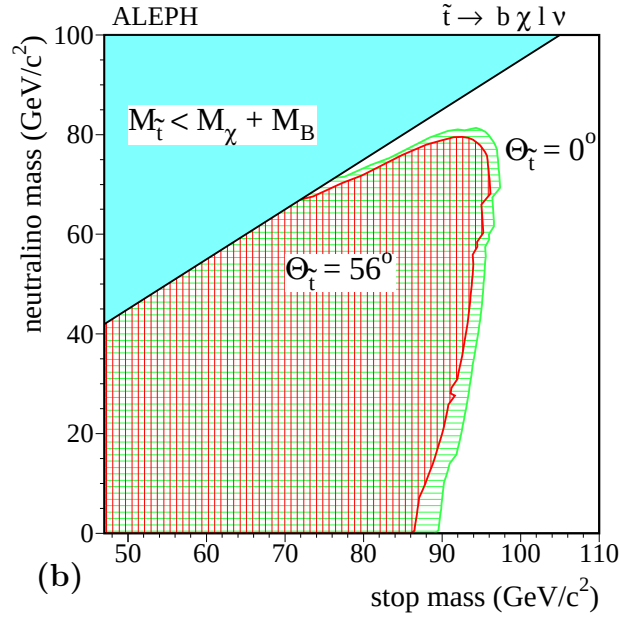
Figure 3: Excluded regions at 95% C.L. in the M_{\chi} vs M_{\tilde{t}} plane from \tilde{t} \rightarrow b \chi \bar{f} f' searches: (a) the W^* modes or (b) the leptonic modes are assumed to be dominant for the \bar{f} f' final states. The excluded regions are given for \theta_{\tilde{t}} = 0^\circ , corresponding to maximum \tilde{t} \tilde{t} Z coupling, and for \theta_{\tilde{t}} = 56^\circ , corresponding to vanishing \tilde{t} \tilde{t} Z coupling.
