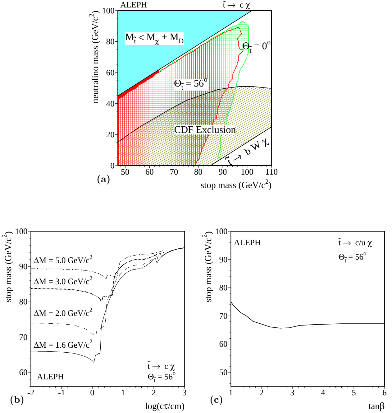
Figure 2: (a) Excluded regions at 95% C.L. in the M_\chi vs M_{\tilde{t}} plane from \tilde{t} \rightarrow c/u\chi searches; the excluded regions are given for \theta_{\tilde{t}} = 0^\circ , corresponding to maximum \tilde{t}\tilde{t}Z coupling, and for \theta_{\tilde{t}} = 56^\circ , corresponding to vanishing \tilde{t}\tilde{t}Z coupling. The dark region in the small \Delta M corridor is excluded by the “long-lived hadrons” analysis. The CDF experiment result is also indicated. (b) Stop mass lower limit at 95% C.L. from the “long-lived hadrons” as a function of \log(c\tau_{\tilde{t}}/\text{cm}) for several \Delta M values, without any assumption on the relation between \Delta M and the stop lifetime \tau_{\tilde{t}} . (c) Stop mass lower limit at 95% C.L. from the “long-lived hadrons” analysis as a function of \tan\beta , independent of the other MSSM parameters.
