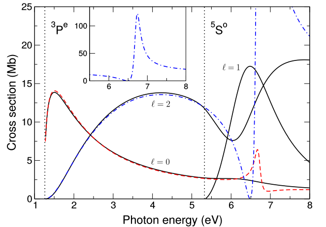
FIG. 5. Theoretical partial photodetachment cross sections as a function of the photon energy, length form. Full lines: full calculation, final channels C(^3P) + e^- (\ell = 0, 2) and C(^5S^o) + e^- (\ell = 1) ; dashed line: without C(^5S^o) , final channel C(^3P) + e^- (\ell = 0) ; dashed-dot line: without C(^5S^o) , final channel C(^3P) + e^- (\ell = 2) . Vertical dotted lines: positions of the C(^3P) and C(^5S^o) thresholds in the R -matrix calculations.
