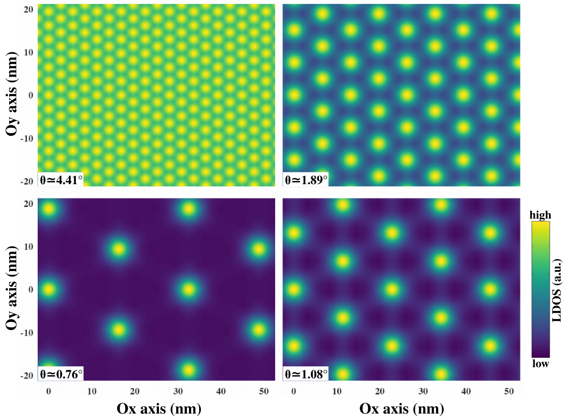
Figure 4. Real-space LDOS images in TBLG at different twist angles. Energy is fixed where the strongest electronic localization is obtained, i.e. at the van Hove singularity point in DOS (see figure 3) for \theta > 1.1^\circ and at zero energy for \theta \lesssim 1.1^\circ .
