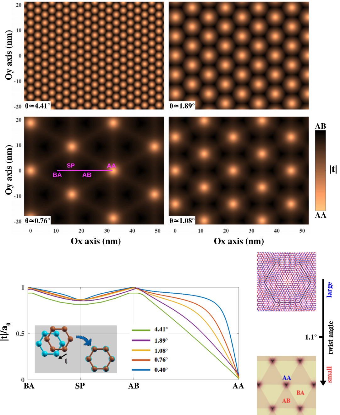
Figure 2. Stacking structure of TBLG imaged by the spatial variation of stacking vector \mathbf{t} (as defined in the inset of bottom-left panel) when varying the twist angle \theta . Four top images are 2D real-space representation of |\mathbf{t}| while the bottom-left one is a plot of |\mathbf{t}| extracted along the line connecting BA–SP (soliton line)—AB–AA stacking regions. The bottom-right diagram is a simple description of the stacking properties of TBLG in the different \theta -regimes (from large to small twist-angles).
