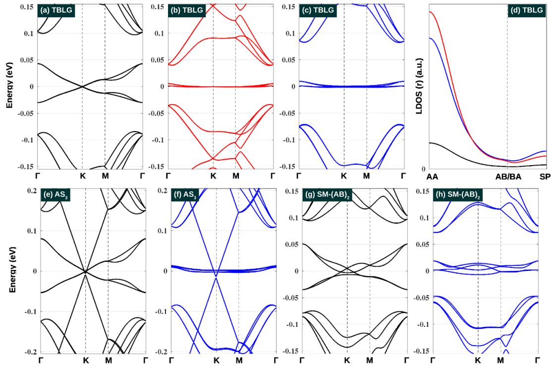
Figure 15. Electronic structures of TMGs modulated by strain and vertical pressure. TBLG at \theta \simeq 1.30^\circ is considered in (a) for the pristine case, in (b) with a biaxial strain of 9%, and in (c) with a vertical pressure P \simeq 1.45 GPa. The corresponding LDOS obtained at the strongest electronic localization point is presented in (d). Electronic bandstructures of AS_3 at \theta \simeq 1.89^\circ with P = 0 and \simeq 2.27 GPa is displayed in (e) and (f), respectively. The results of SM-(AB)_2 at \theta \simeq 1.47^\circ with P = 0 and \simeq 2.27 GPa are in (g) and (h), respectively.
