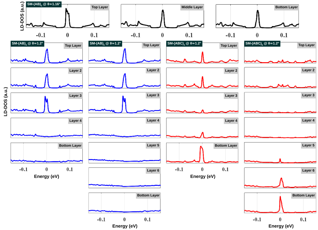
Figure 7. Layer decomposed DOS (LD-DOS) in some SM-systems considered in figure 5.
