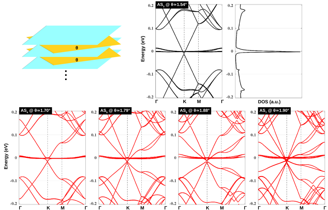
Figure 8. Electronic bandstructures of alternatively twisted systems of graphene monolayers schematized on top-left (i.e. the AS_n systems specified in figure 1) with \theta near their magic angle \theta_n^{MA} (see text). On top-right, DOS versus energy in AS_2 -structure is also superimposed.
