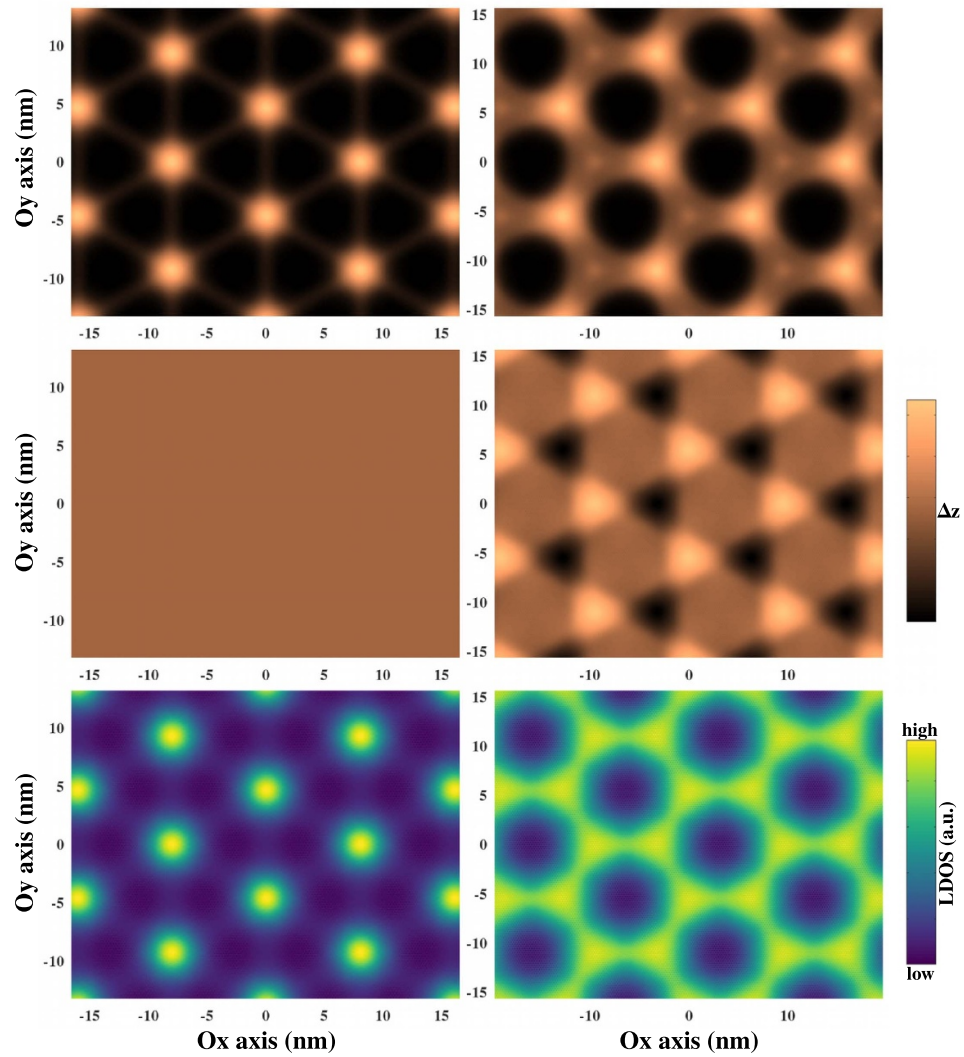
Figure 11. The structural and electronic properties of two AS_3 structures: AS_3 at \theta \simeq 1.54^\circ in figure 8 (see in the left) and AS_3 at \theta \simeq 1.30^\circ considered in figure 10(a) (see in the right). Images in the first and second rows present the spatial variation of out-of-plane displacements in the top and middle layers, respectively. LDOS of two systems at zero energy is presented in the bottom images.
