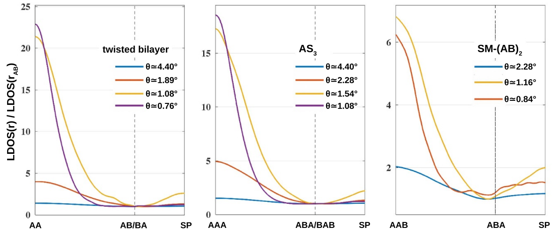
Figure 14. Spatial variation of LDOS in TBLG, AS_3 and SM-(AB)_2 systems when varying the twist angle around their magic one. The presented LDOS is extracted along the line connecting regions where AA, SP, AB/BA stacking configurations occur. Calculations are performed at energy where the strongest electronic localization is obtained, i.e. at the electron van Hove singularity point for large \theta and at zero energy for \theta below the magic angle.
