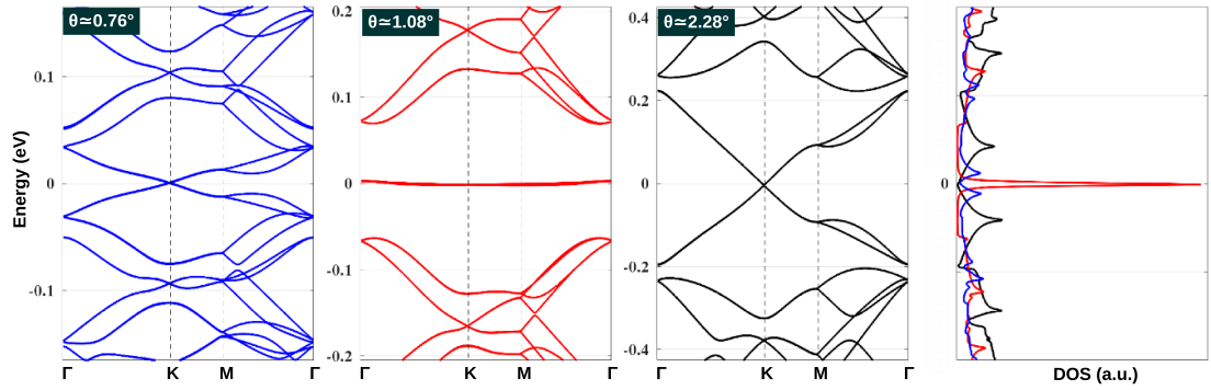
Figure 3. Electronic bandstructure of TBLG for the twist angle \theta < 1.1^\circ (left in blue), \theta \simeq 1.1^\circ (center in red) and \theta > 1.1^\circ (right in black). The corresponding density of states (DOS) are presented on the extreme right with the same color scale for the three moiré structures.
