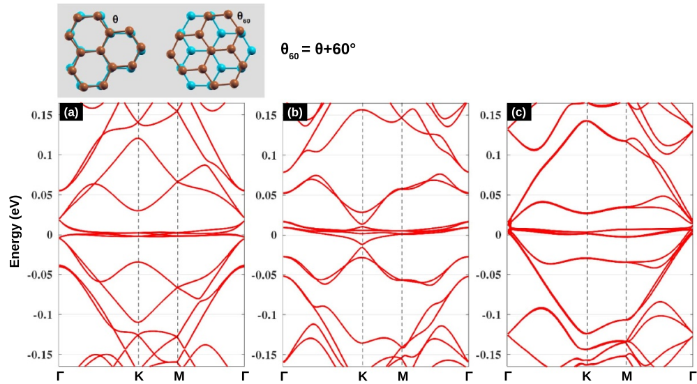
Figure 10. Electronic bandstructures of AS_n systems when one or a few layers are additionally rotated by 60^\circ (see the illustration on top). In (a) and (b), the top layer of AS_3 at \theta \simeq 1.30^\circ and AS_4 at \theta \simeq 1.54^\circ , respectively, is additionally rotated by 60^\circ . In (c), such additional 60^\circ -rotation is applied to two top layers of AS_4 at \theta \simeq 1.35^\circ .
