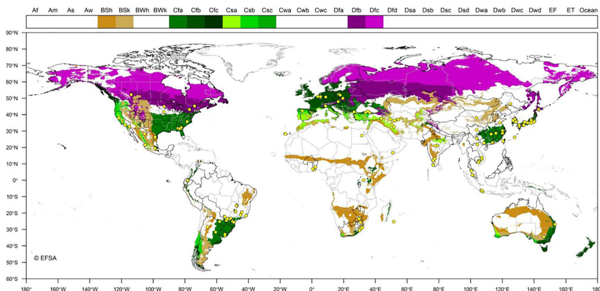
Figure 2: Distribution of Köppen-Geiger climate types BSh, BSk, Cfa, Cfb, Csa, Csb, Csc, Dfb and Dfc that occur in the EU and in third countries where P. ananatis has been reported. The legend shows the list of Köppen-Geiger climates. Yellow dots indicate point locations where P. ananatis was reported (Appendix B)
