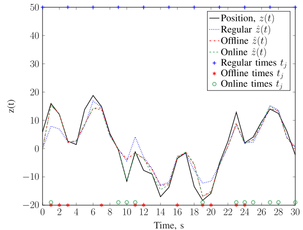
Fig. 7. Comparison of a particular realization z(t) with the filtered values \hat{z}(t) obtained with a particle filter with regular measurement times and both the offline and the online particle filters. The gains on the complete sequence are G_{\text{offline}} = 0.173 and G_{\text{online}} = 0.283 . Results are simulated from the common benchmark (Subsection III-A2).
