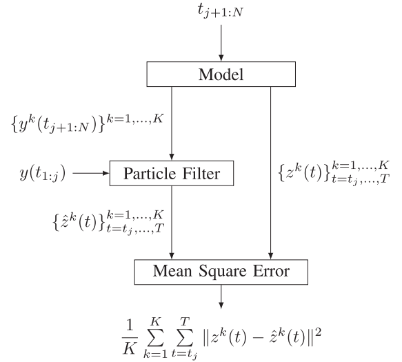
Fig. 2. Representation of the Monte Carlo algorithm that estimates \mathbb{E}_{y(t_{j+1:N})}[\sum_{t=t_j}^T \mathcal{E}[t; y(t_{1:N})]] . The outputs generated by the Model block are drawn according to (1) through (4) and the distributions of v(t) and w(t) . The particle filter computes an estimate \hat{z}^k(t) = \hat{z}^k(t; y(t_{1:j}), y^k(t_{j+1:N})) of z^k(t) from previous intermittent measurements. The Mean Square Error block computes the mean squared of the difference between its inputs; it is the right-hand side of (15).
