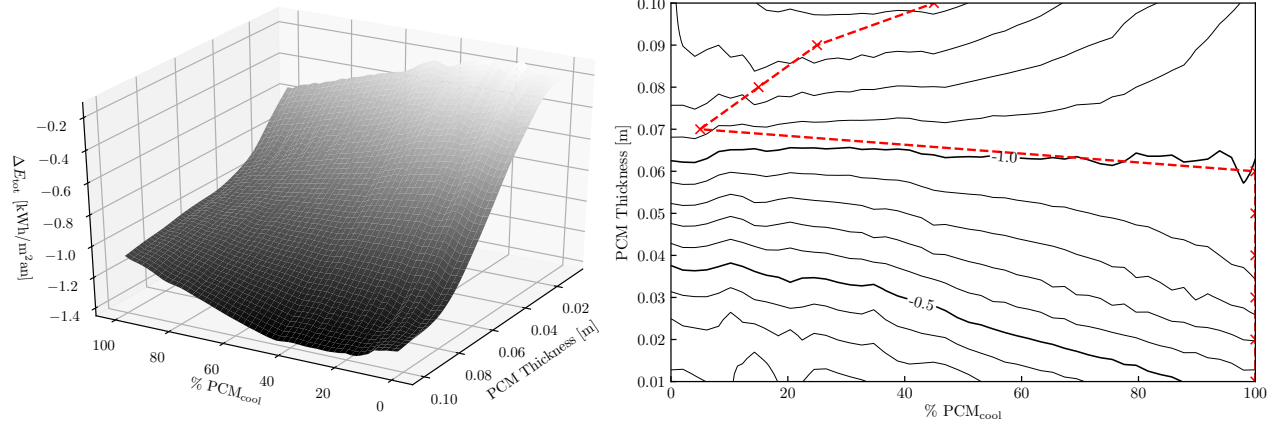
(a) Configuration \text{PCM}_{\text{cool}} // \text{PCM}_{\text{heat}} .
