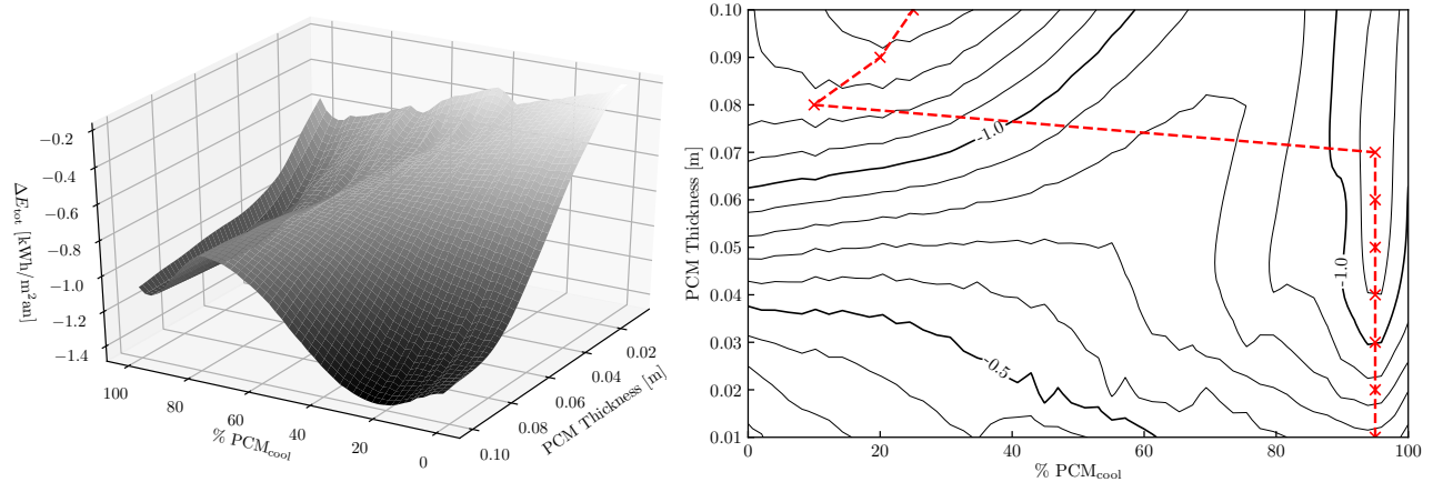
(c) Configuration \text{PCM}_{\text{heat}} -- \text{PCM}_{\text{cool}}
