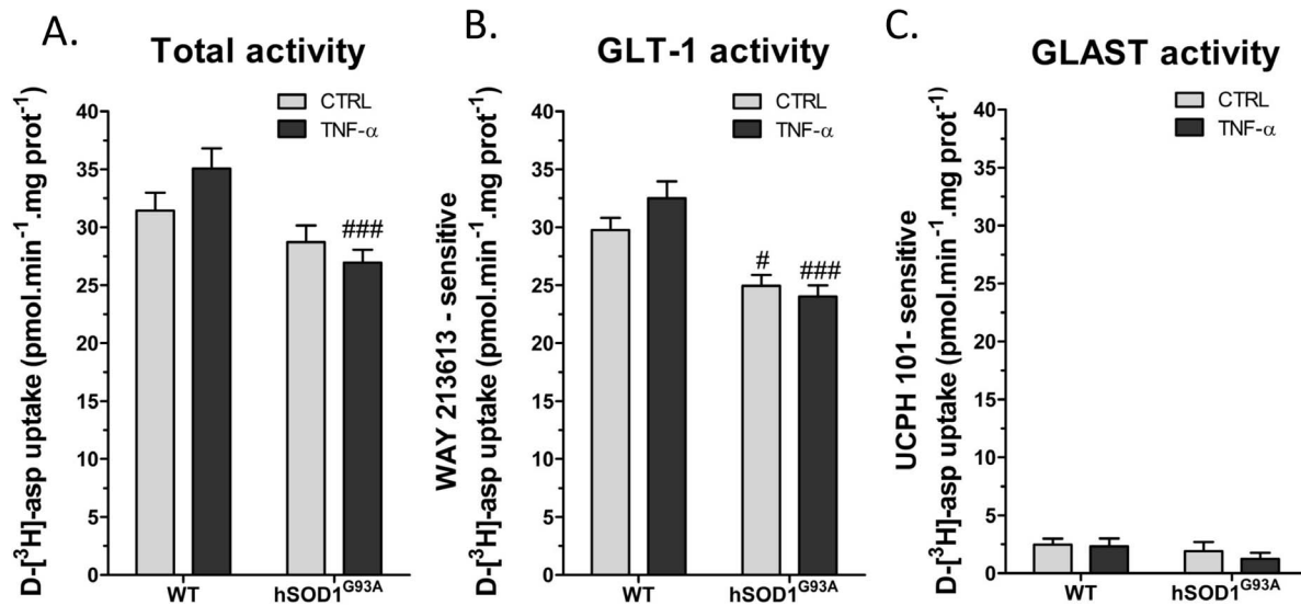
Figure 4. Influence of TNF- \alpha on the activity of glutamate transporters from wild-type or hSOD1 G93A cortical astrocytes. Glutamate transporter activity was evaluated by measuring velocity of D-[ 3 H]-aspartate uptake (50 nmol/L) in wild-type and hSOD1 G93A astrocytes treated or not with TNF- \alpha (20 ng/mL) for 72 h. (A) shows total uptake while (B) and (C) illustrate GLT-1- and GLAST-dependent uptake, respectively evaluated in presence of the selective inhibitors WAY-213613 (100 \mu mol/L) and UCPH-101 (10 \mu mol/L). Shown are mean with SEM from five independent experiments realized in quintuplicate. # p <0.05 and ### p <0.001 for comparison between different genotypes with the same treatment. doi:10.1371/journal.pone.0097649.g004
