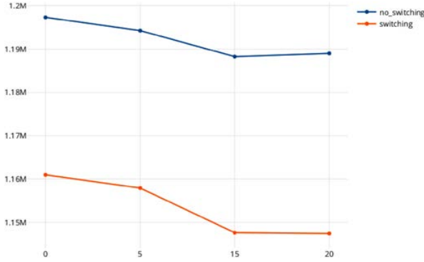
Fig. 4. Evolution of the average hourly total cost on the 32 snapshots, as a function of the size of the set U_{prev} in the N-1 case. “no_switching” refers to the case of a cost-minimizing real-time model without switching, while “switching” corresponds to reactive switching.
