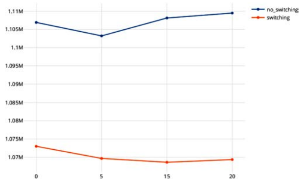
Fig. 3. Evolution of the average hourly total cost on the 32 snapshots, as a function of the size of set U_{\text{prev}} in the N case. “no_switching” refers to the case of a cost-minimizing real-time model without switching, while “switching” corresponds to reactive switching.
