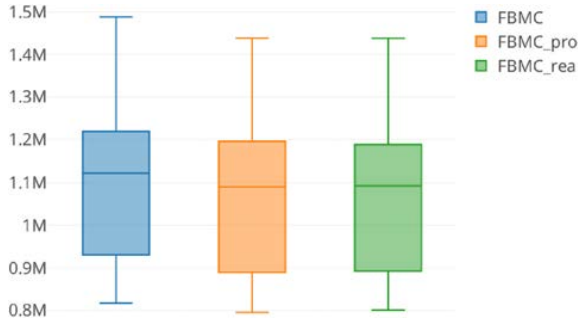
Fig. 2. Hourly total cost of the different cases studied on 32 snapshots of CWE. “FBMC” refers to the case of a cost-minimizing real-time model without switching. The suffix “_rea” is for reactive (day-ahead) switching, “_pro” is for proactive (day-ahead and real-time) switching.
