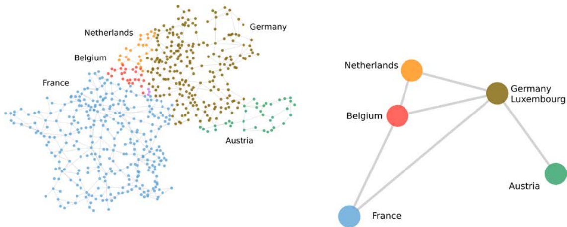
Fig. 1. The CWE network model (left) and its zonal aggregation (right).
