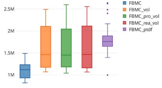
Fig. 8. Hourly total cost of the different re-dispatch and balancing methods on 32 snapshots of CWE. In this figure, the “FBMC” series refers to the same series as the “FBMC” series of Fig. 2, i.e. a cost-minimizing real-time model without switching. The suffix “_vol” is for the volume-minimizing real-time model, “_ptdf” is for the PTDF-based heuristic. Note that, for the latter, there is no switching action possible, as it is based on the PTDF obtained for a reference topology.
