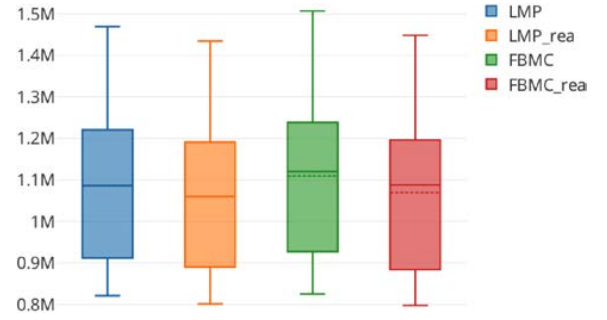
Fig. 5. Hourly total cost of the different cases studied on 32 snapshots of CWE in the N case. “FBMC” refers to the case of a cost-minimizing real-time model without switching. The suffix “_rea” is for reactive switching.
