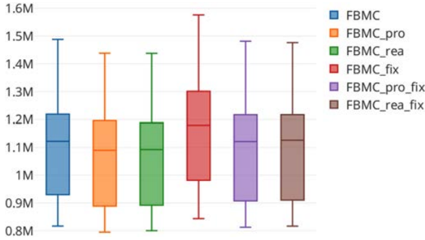
Fig. 7. Hourly total cost of the different cases that are studied on 32 snapshots of CWE. The suffix “_fix” refers to the case where the net positions are fixed to their day-ahead values.
