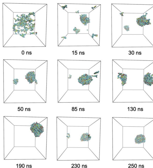
Fig. 2 Snapshots of the simulation box showing supramolecular aggregation over time for NP7. Water molecules are not displayed. A video of the time-evolution of the aggregation is provided in the ESI † .
