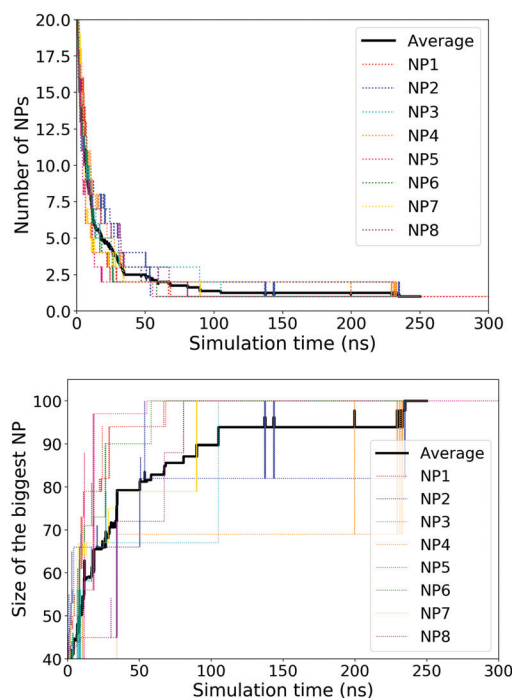
Fig. 3 Evolution of the number of NPs (top) and of the size of the biggest NP (bottom) with simulation time for the 8 replicated MD simulations. Abrupt increases in the evolution are due to the coalescence of two "large" aggregates. Two molecules are considered to be in the same aggregate if at least a couple of non-hydrogen atoms are closer than 4.0 Å.
