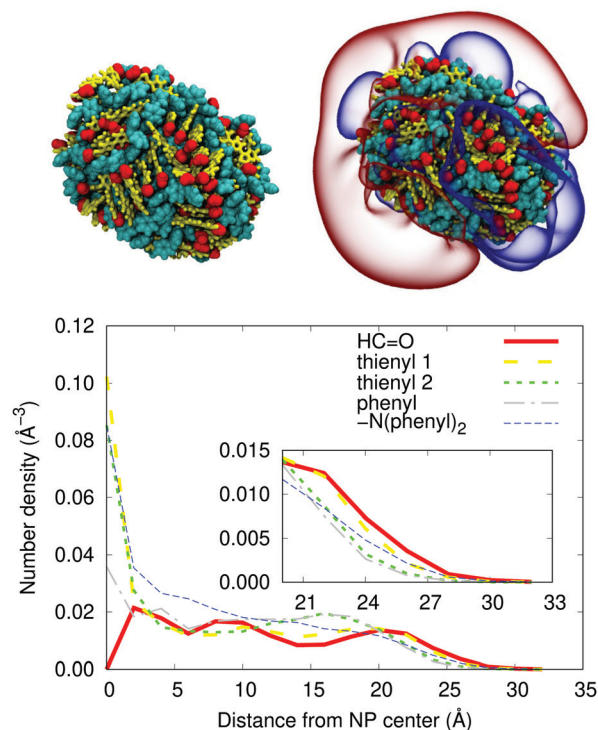
Fig. 4 Top left: Example of ellipsoidal nanoparticles composed of 100 aggregated dyes highlighting the orientation of formyl groups (in red) towards the outside, and the \pi -stacked domains (in yellow); top right: electrostatic potential calculated from the atomic charge distribution (isovalues range from -4 (blue) to +4 (red), in kT/e units, with T = 300 K); bottom: radial number density of the different molecular moieties as a function of the distance from the center of the nanoparticle. Values averaged over 100 molecules of the 8 final nanoparticles (NP1–NP8).
