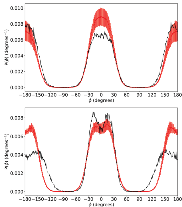
Fig. 5 Distribution of the \phi_{TT} (top) and \phi_{TP} (bottom) dihedral angles (Fig. 1) for a single dye in water solution (in black, monitored over 1000 ns) and embedded into a nanoparticle (in red, averaged for the 100 constitutive dyes of the 8 final NPs, over the last 50 ns; standard deviations are also displayed).
