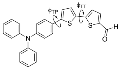
Fig. 1 Chemical structure of the dipolar dye investigated in this work, with the dihedral angles \phi_{TT} = \text{S}-\text{C}-\text{C}-\text{S} and \phi_{TP} = \text{C}-\text{C}-\text{C}-\text{S} .
