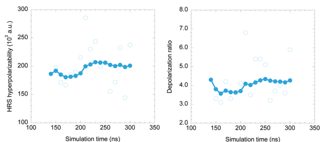
Fig. 9 Time evolution of \beta_{\text{HRS}} (left) and DR (right) values for NP5 (empty dots) and of their cumulative moving averages (full dots), as calculated using the tensor-sum approximation at the TD-DFT:M06-2X/6-311+G(d) level.
