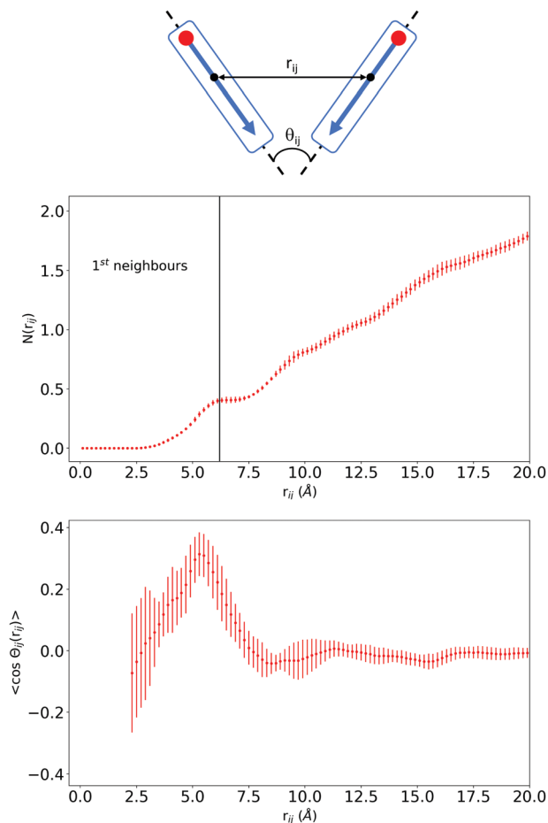
Fig. 7 Definition of the angle \theta_{ij} between molecular dipoles and the distance r_{ij} , between molecular centers of mass (top), and evolution of the mean density of neighbours N(r_{ij}) (middle) and of the mean cosine of \theta_{ij} (bottom) as a function of r_{ij} . Standard deviations obtained from averaging the results of the 8 NPs are also displayed.
