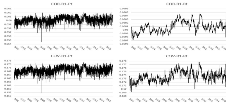
Figure 1 Time series of a_{ij,t} coefficients estimated with the COR-R1-Pt and the COR-R1-Rt models (upper graphs) and with the COV-R1-Pt and the COV-R1-Rt models (lower graphs). The coefficients are for the asset pair AXP–JPM.
