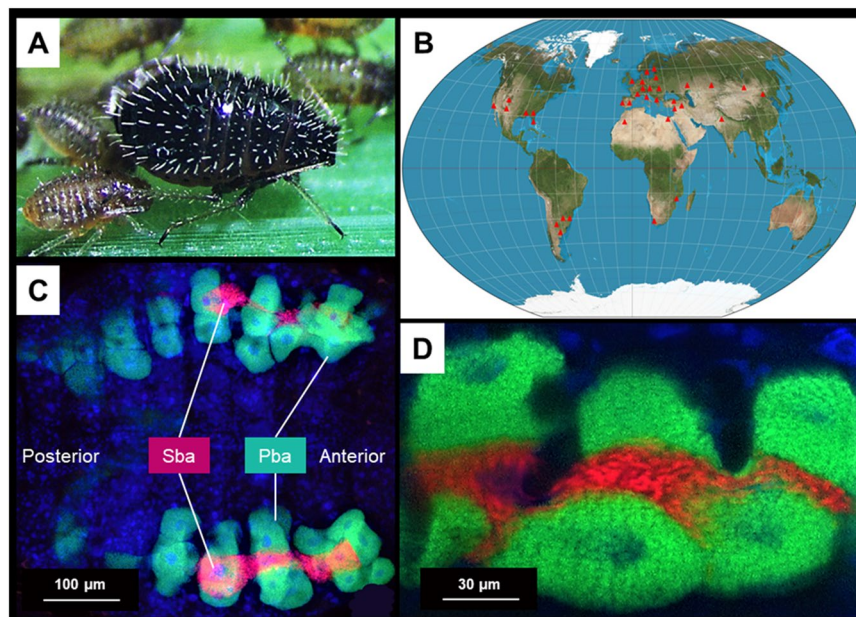
Fig. 1 The cereal aphid Siphia maydis and its di-symbiotic system. (A) An adult surrounded by several nymphs, all feeding on bread wheat, Triticum aestivum . (B) Distribution of S. maydis worldwide. Red triangles represent collection locations reported in the literature. (C) Serratia symbiotica (red) is compartmentalized into syncytial secondary bacteriocytes (Sba) sandwiched between the uninucleate primary bacteriocytes (Pba) housing Buchnera aphidicola (green), forming a horseshoe-shaped bacteriome (green, red, and blue signals indicate B. aphidicola cells, S. symbiotica cells and host insect nuclei, respectively). (D) Close-up view of primary and secondary bacteriocytes showing their embedded layout.
