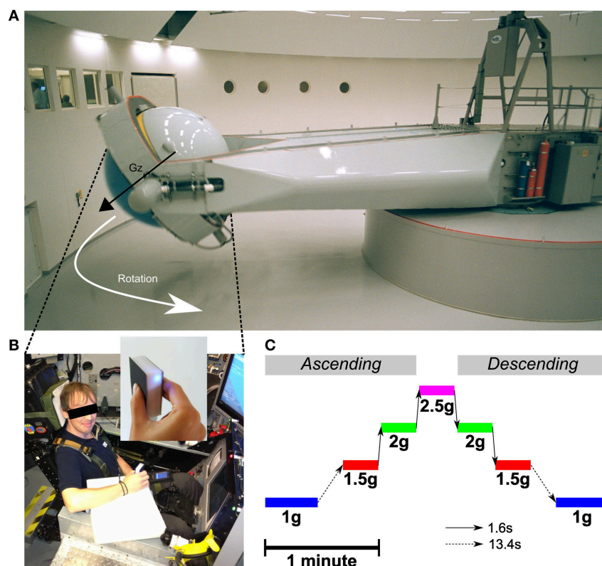
FIGURE 1 | (A) Centrifuge room and the long-radius (9.1 m) Human Centrifuge operated by QinetiQ. The control room can be seen through the windows on the left. The vector G_z illustrates the direction of the gravito-inertial force. (B) Subject seated in the training insert cockpit mock-up in the gondola. The manipulandum (see enlargement) was held in the right hand and was connected to a palm pilot device through a Bluetooth connection. The manipulandum was attached to the wrist and the palm device was strapped to the left thigh. A piece of white foam supported the forearm and ensured the manipulandum was in the same horizontal position between trials. Written informed consent was obtained from the participant on the photo. (C) Time scaled and chronological illustration of the G_z profiles programmed in the centrifuge. The dashed arrow represents the long transition time from and to 1 g (13.4 s) and the solid arrow represents the fast transitions between altered gravito-inertial environments (1.6 s).
