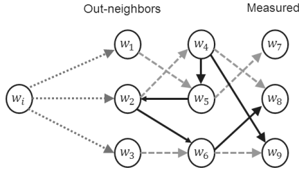
Fig. 5. Example illustrating Corollary 5.2: 3 vertex-disjoint dashed paths to the 3 measured nodes; the 3 dotted edges are identifiable.
