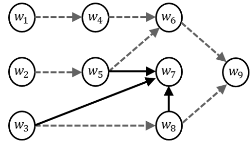
Fig. 6. Example illustrating Theorem 6.1: all transfer functions on the dashed edges can be generically identified from the measurement of node 9.
