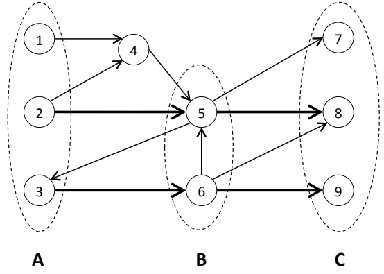
Fig. 4. Illustration of the notions of vertex-disjoint paths, disconnecting sets, and Lemma 5.3. The highlighted paths (2, 5, 8) and (3, 6, 9) are vertex-disjoint paths from \mathcal{A} = \{1, 2, 3\} to \mathcal{C} = \{7, 8, 9\} , and their existence implies b_{\mathcal{A} \rightarrow \mathcal{C}} \geq 2 . An alternative set of such paths is (1, 4, 5, 7) and (3, 6, 9) . On the other hand, every path starting from \mathcal{A} and arriving in \mathcal{C} goes through \mathcal{B} = \{5, 6\} , which is thus an \mathcal{A} - \mathcal{C} disconnecting set. It follows then from Lemma 5.3 that b_{\mathcal{A} \rightarrow \mathcal{C}} \leq 2 and thus that (i) \mathcal{B} is a minimal \mathcal{A} - \mathcal{C} disconnecting set, and (ii) there is no set of more than two vertex-disjoint paths from \mathcal{A} to \mathcal{C} .
